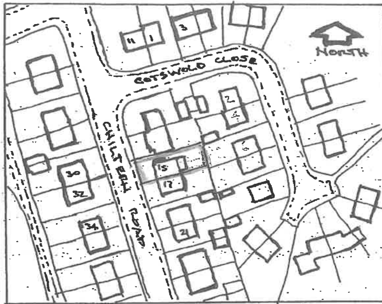
LOCATION PLAN 1:1250
