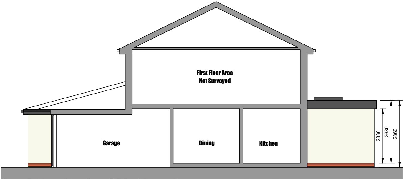
South East Facing Side Elevation
