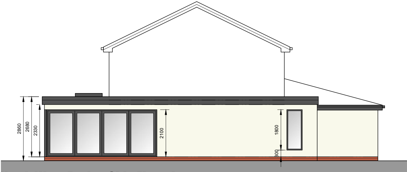
North West Facing Side Elevation
