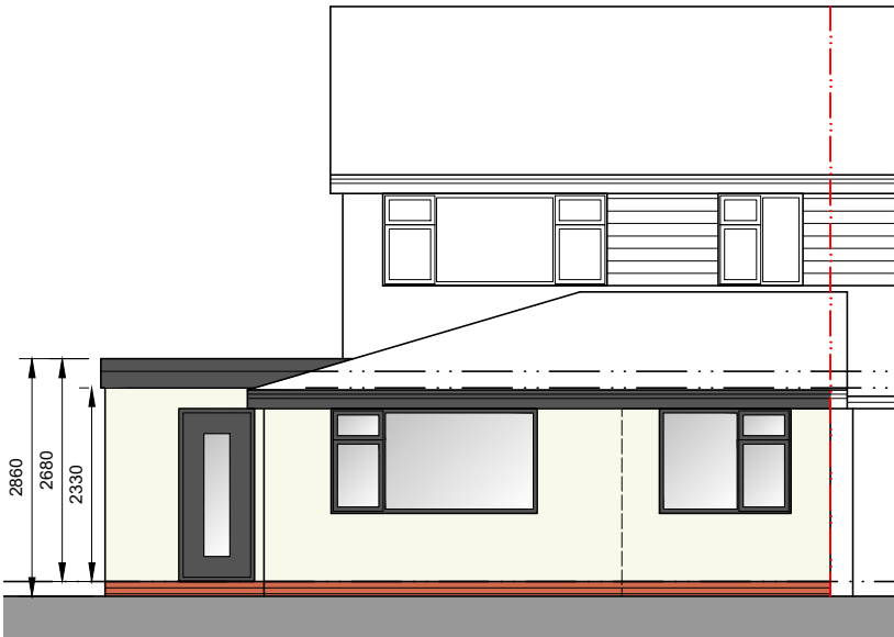
South West Facing Front Elevation
