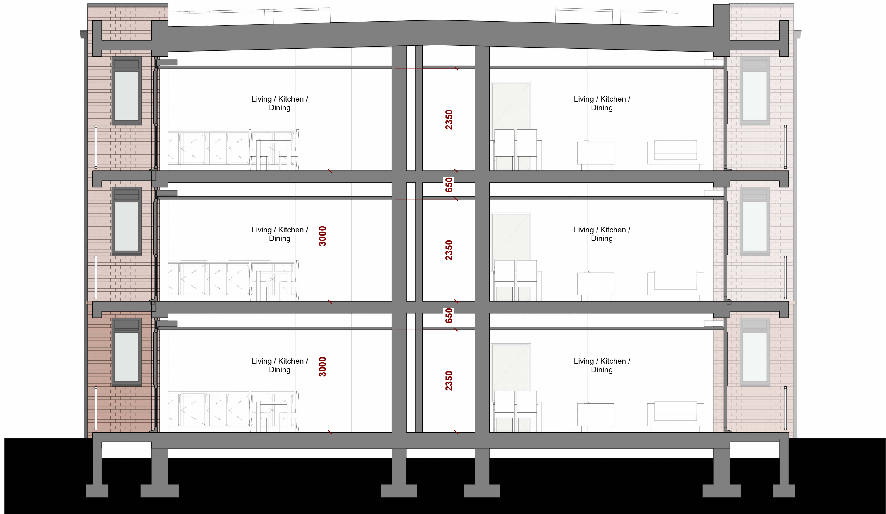
2 Building A Design Section 1 : 50
