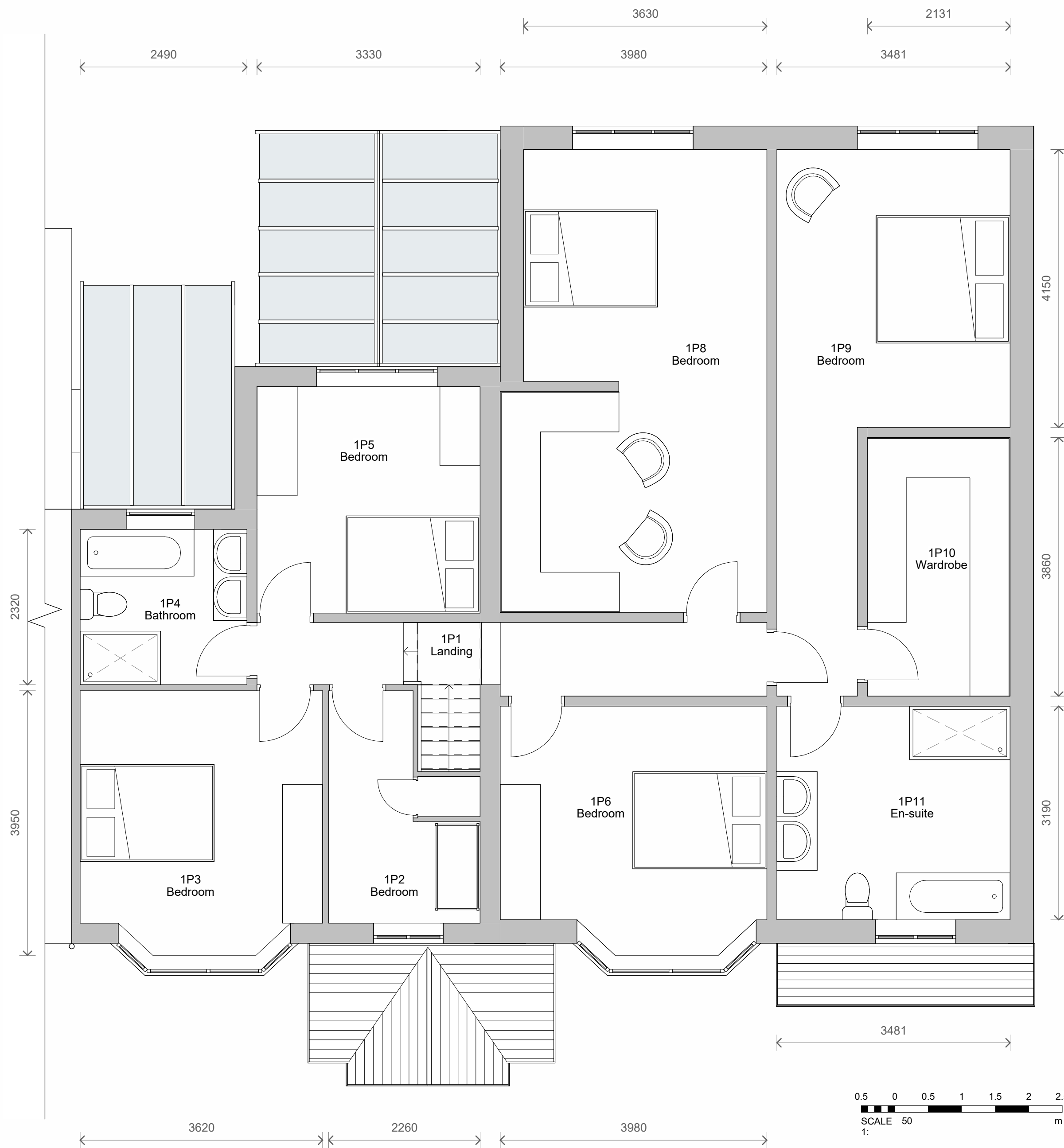
2 Level 1 - Proposed 1 : 50
