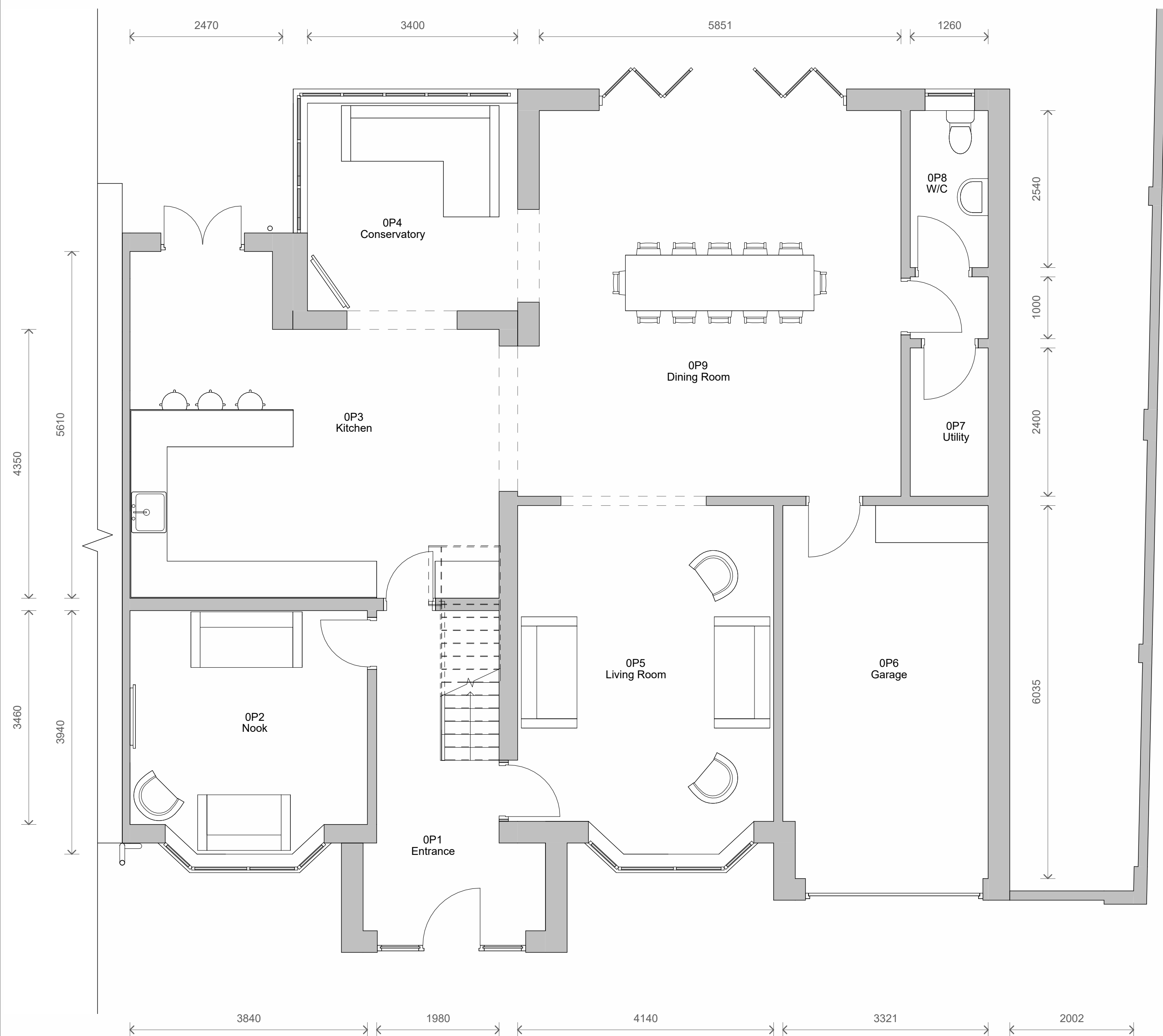
1 Level 0 - Proposed 1 : 50
