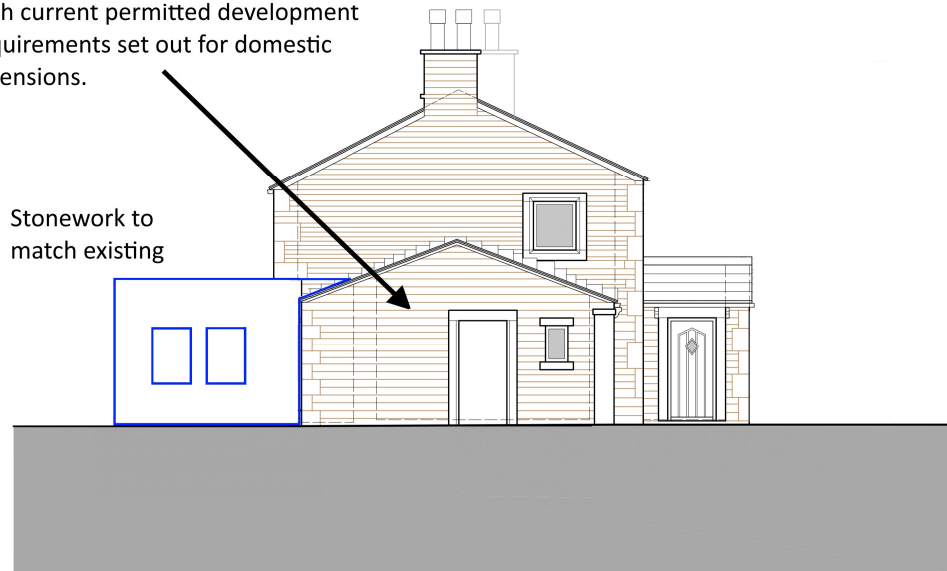
East Elevation
