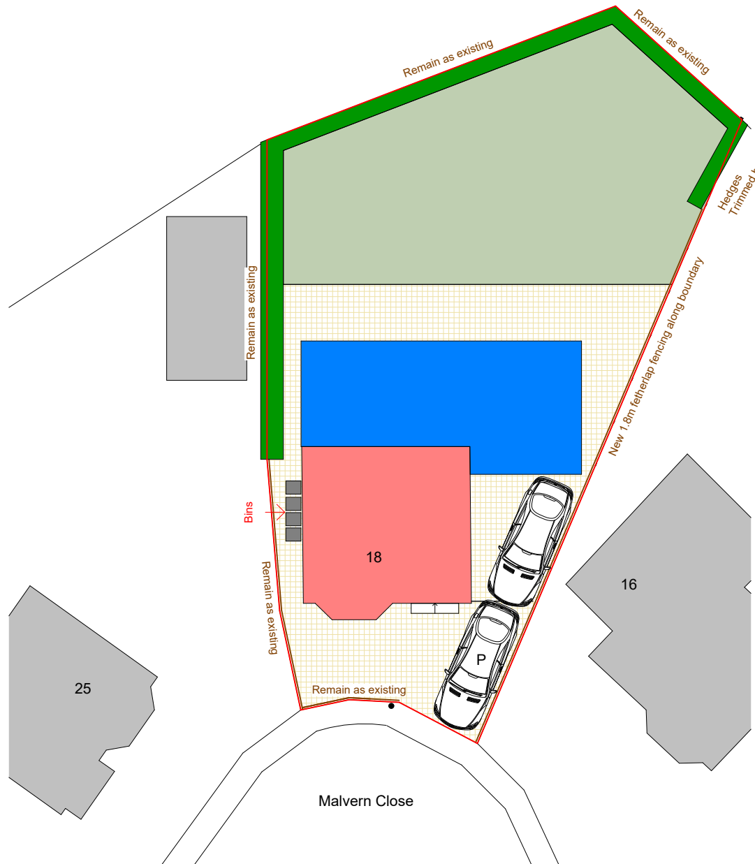
2 Site - Proposed 1 : 200
