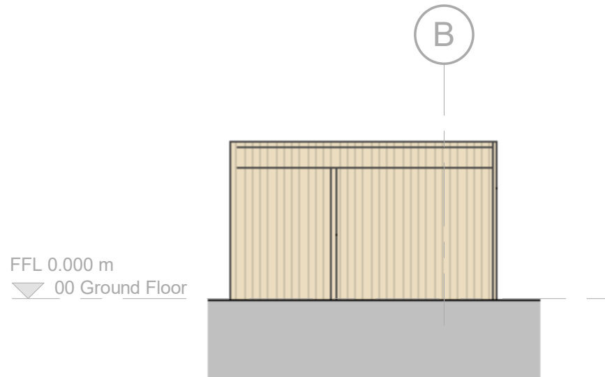
2 Proposed South East Elevation Scale @ 1 : 100
