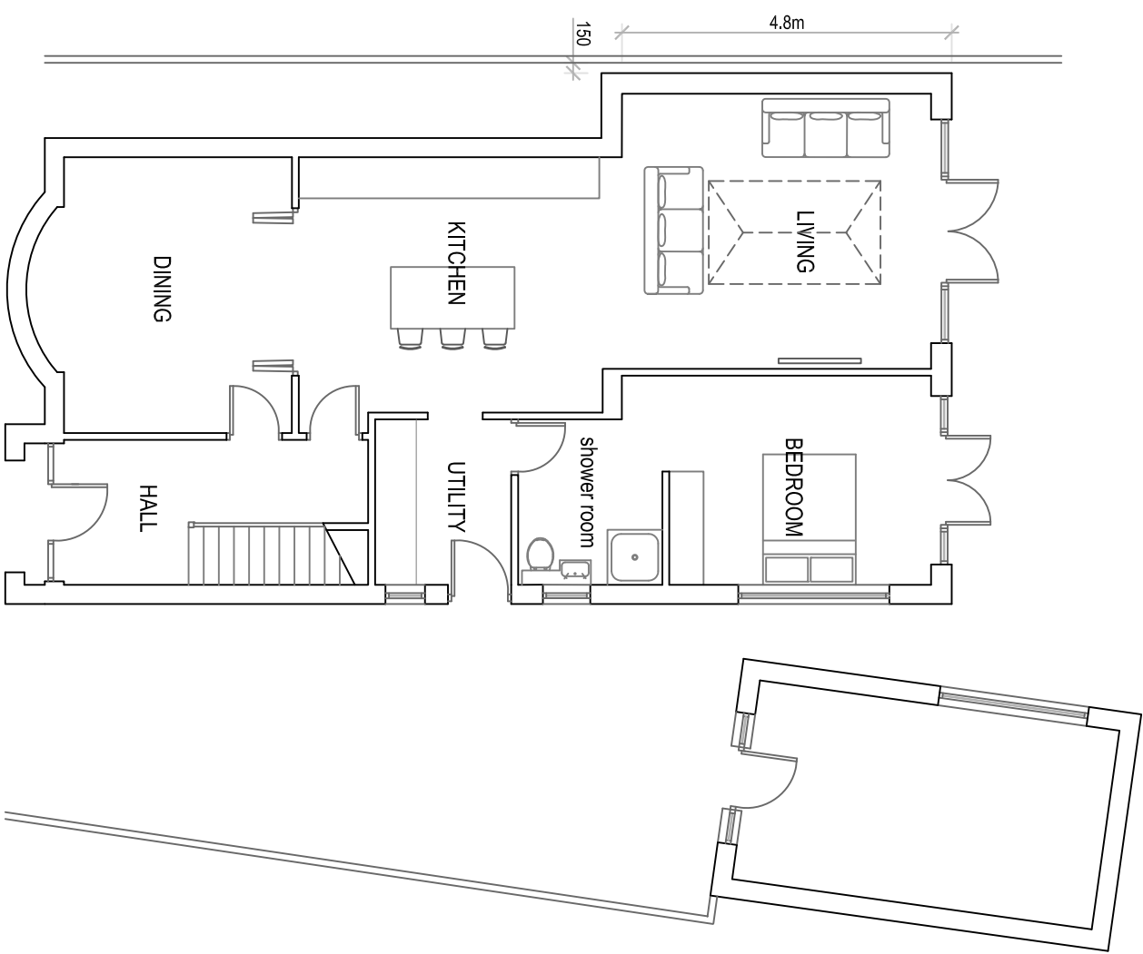
PROPOSED GF PLAN 1:100
