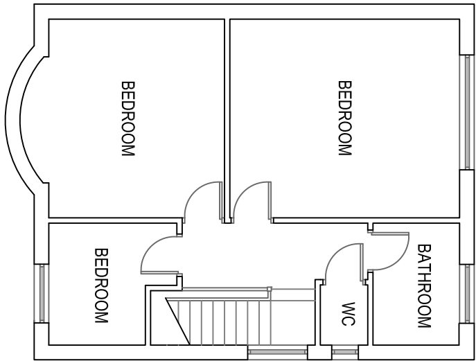
PROPOSED FF PLAN 1:100
