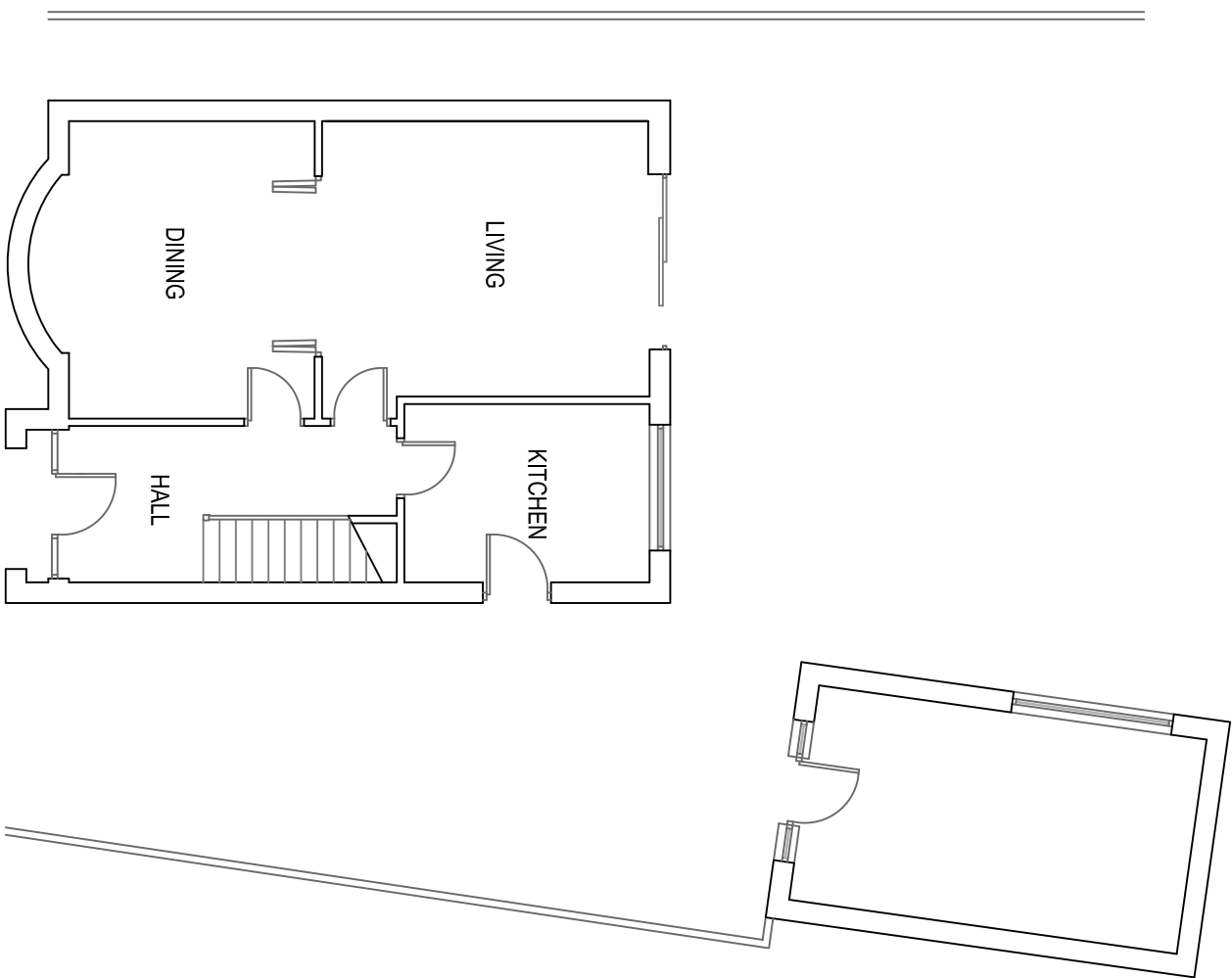
EXISTING GF PLAN 1:100
