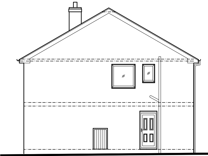
EXISTING SIDE
