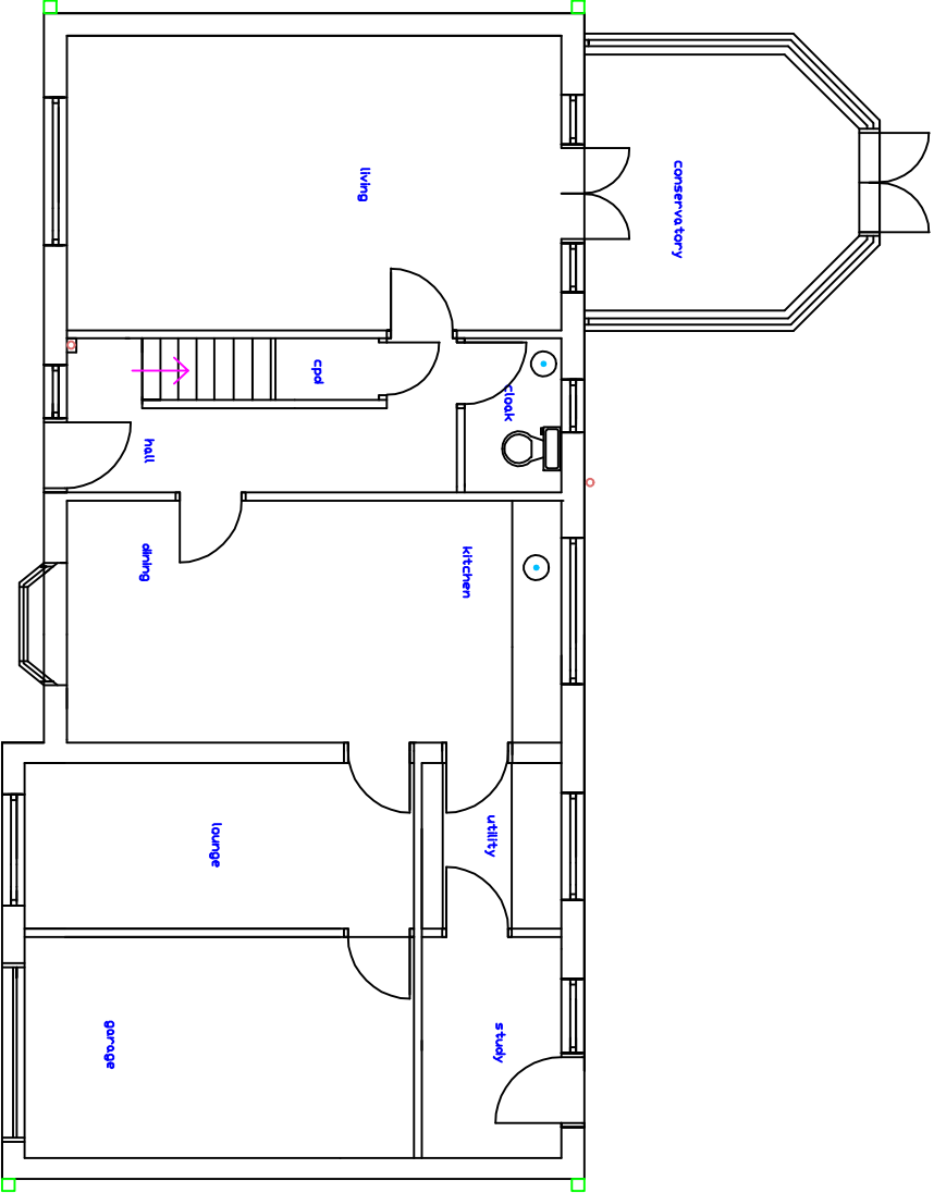
EXISTING GROUND FLOOR 1: 50
