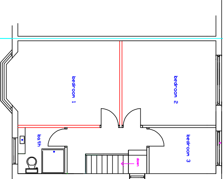
EXISTING FIRST FLOOR LAYOUT 1:100
