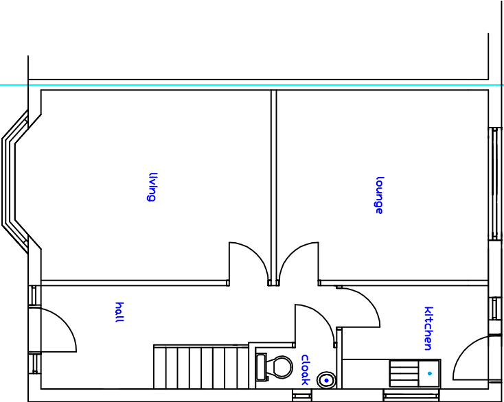
EXISTING GROUND FLOOR LAYOUT 1:100
