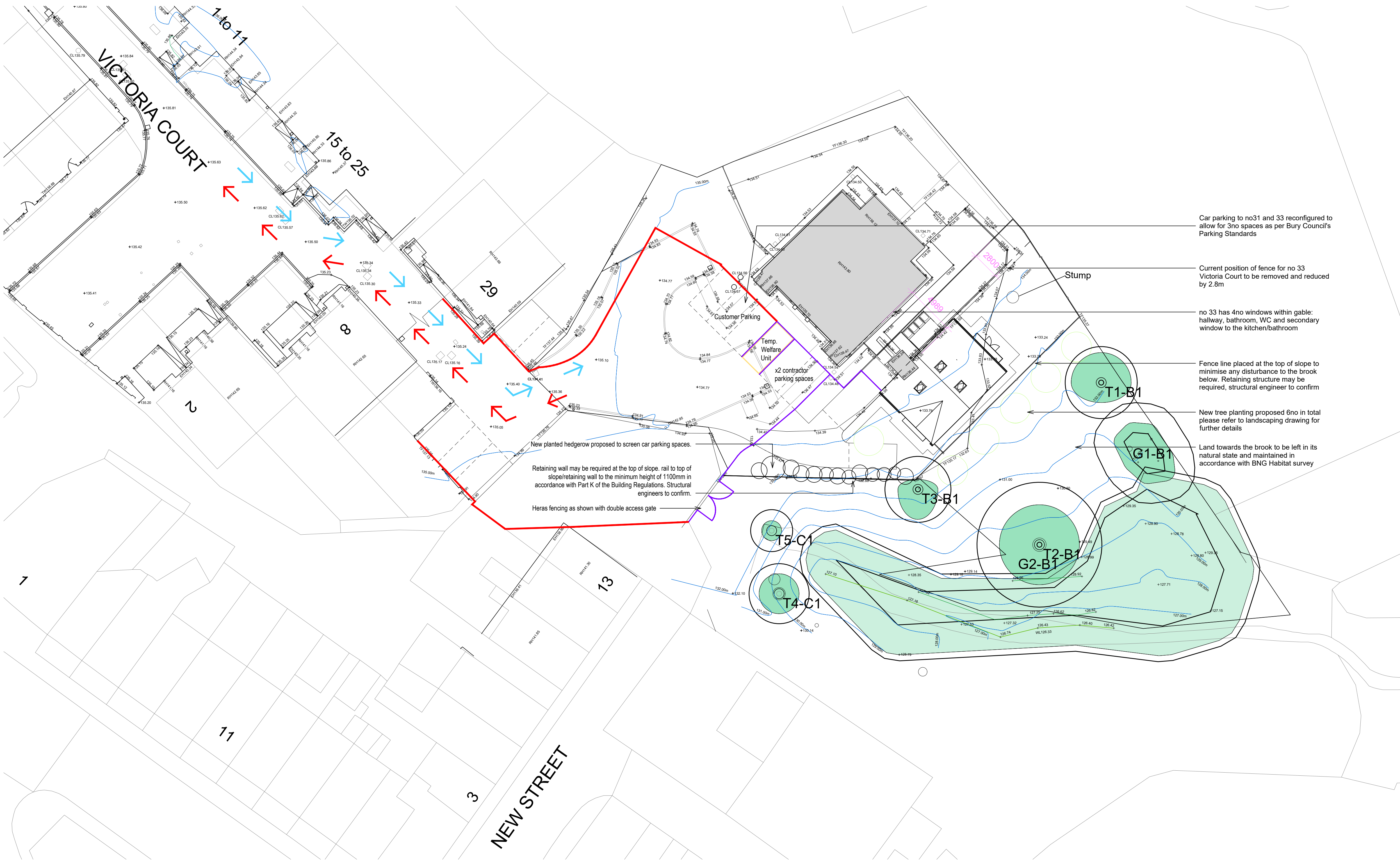
Proposed Site Layout 1:200
