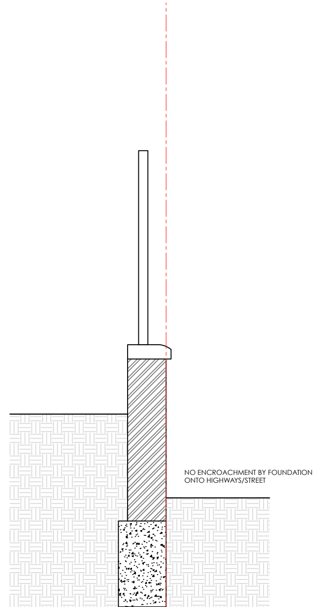
PROPOSED BOUNDARY WALL
