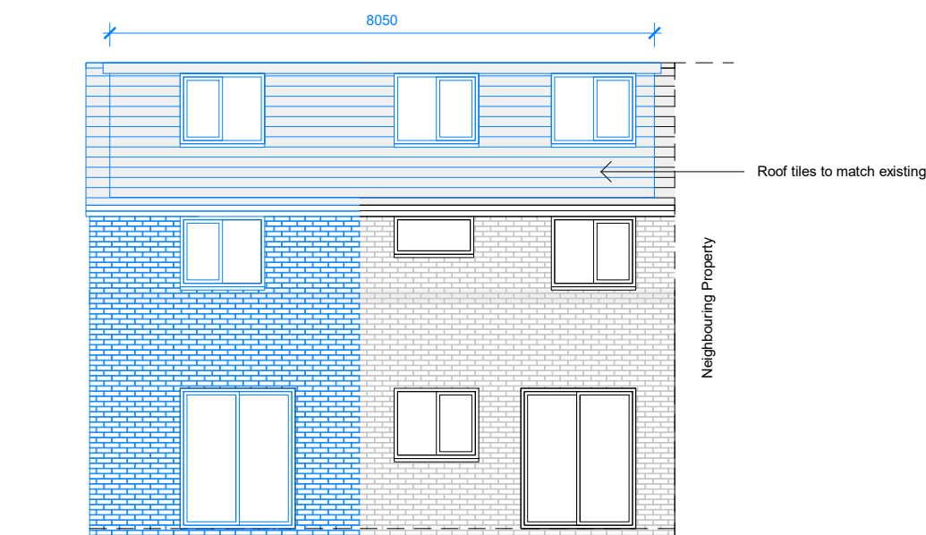
6 Rear Elevation 1 : 100
