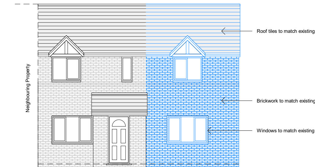
4 Front Elevation 1 : 100
