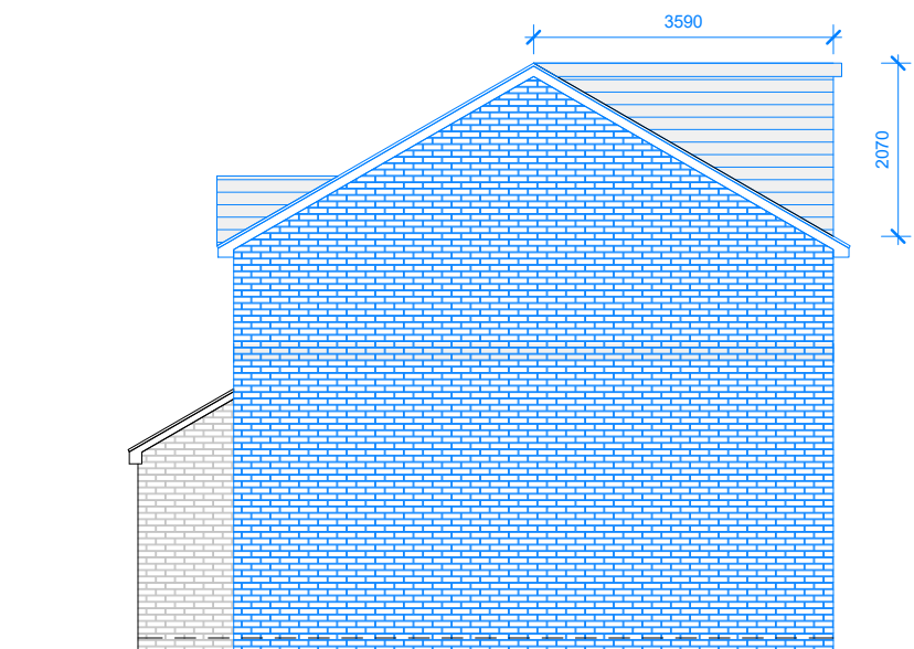
5 Side Elevation (South) 1 : 100
