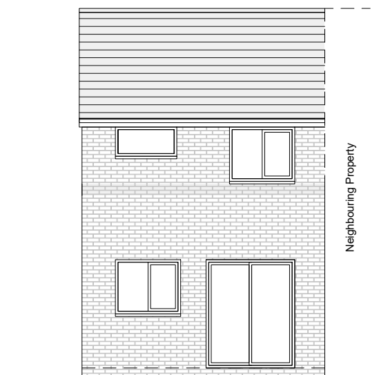
6 Rear Elevation 1 : 100
