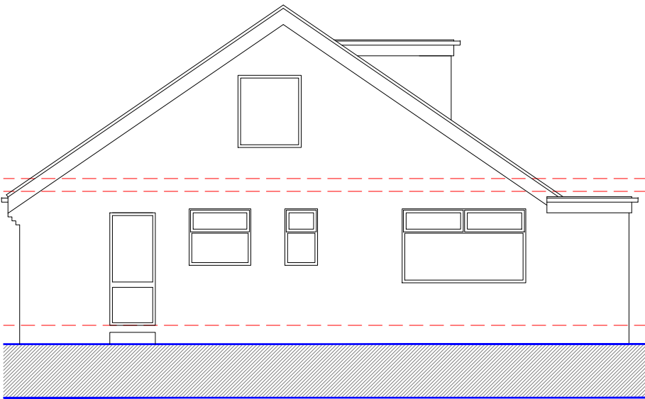
EXISTING GABLE ELEVATION 1:100
