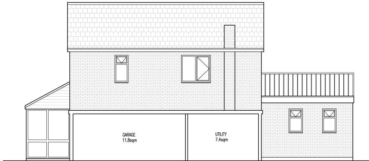
EXISTING SIDE ELEVATION 1:100 @ A3
