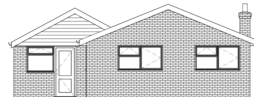
3 Rear Elevation 1 : 100
