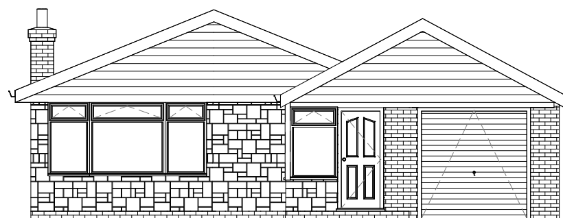
2 Front Elevation 1 : 100
