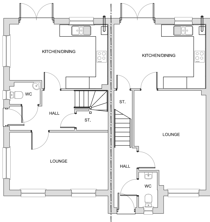
EPSOM (AS) GROUND FLOOR
