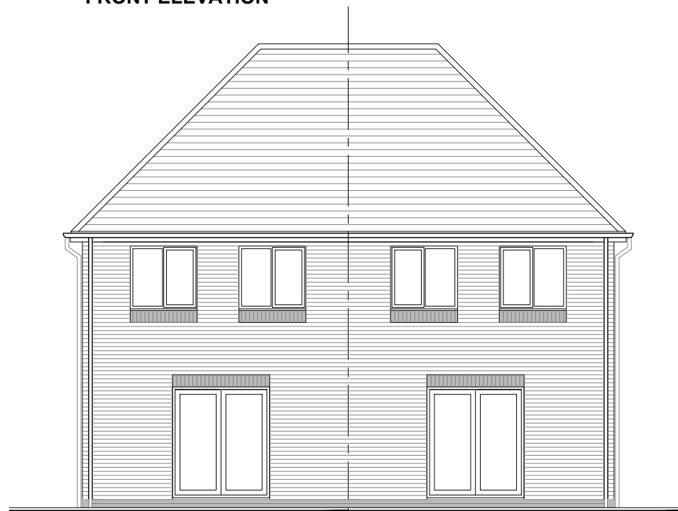
MOXLEY (OPP) REAR ELEVATION
