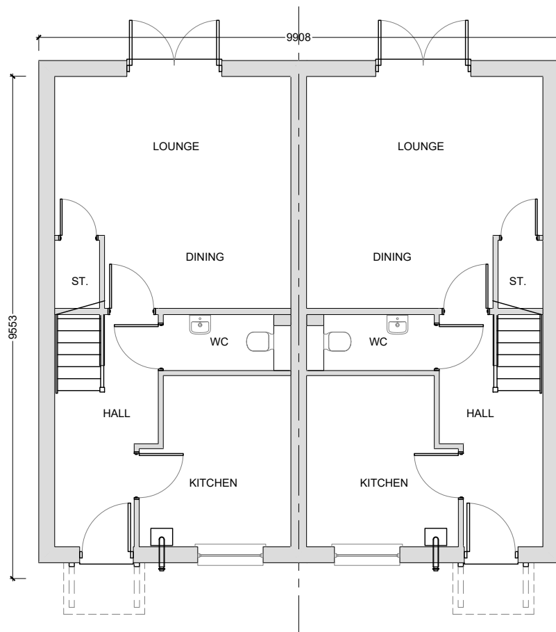
MOXLEY (AS) GROUND FLOOR
