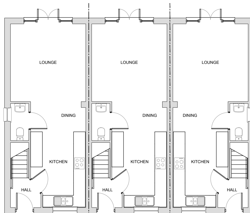
GROUND FLOOR
