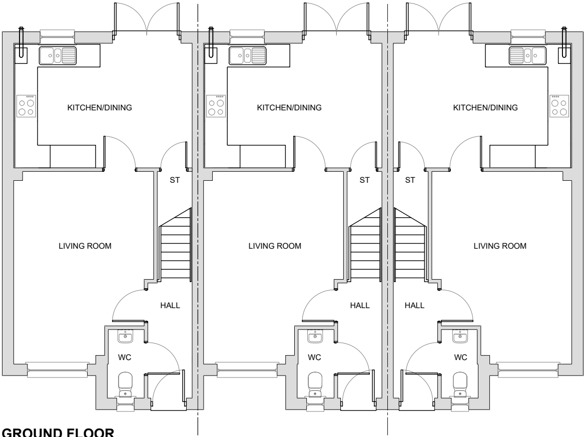
GROUND FLOOR
