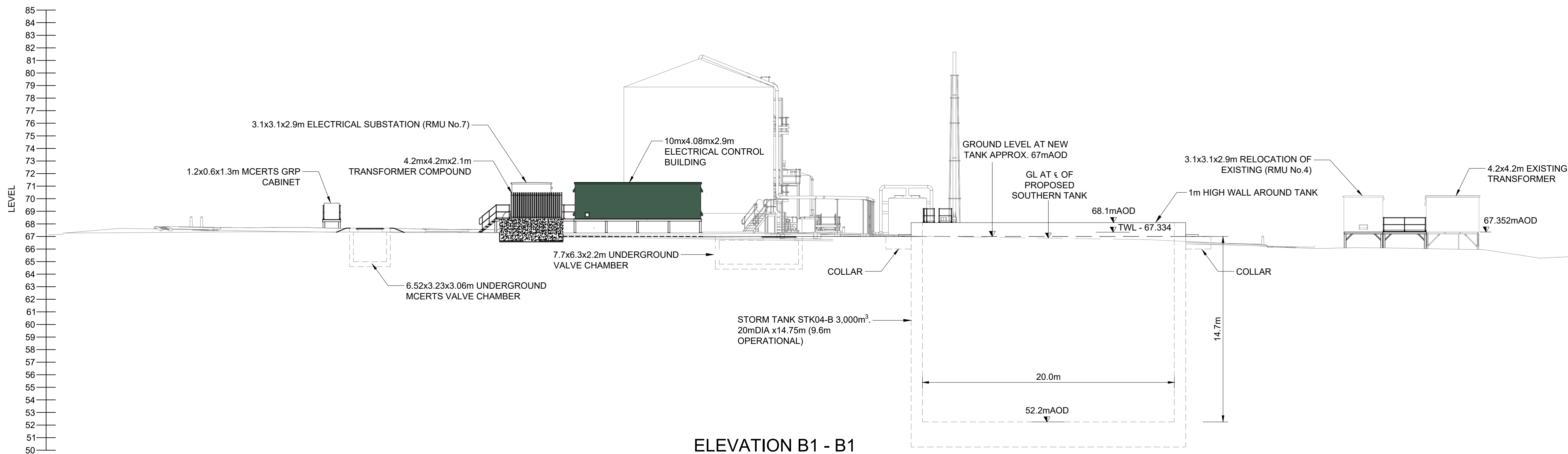
ELEVATION B1 - B1
