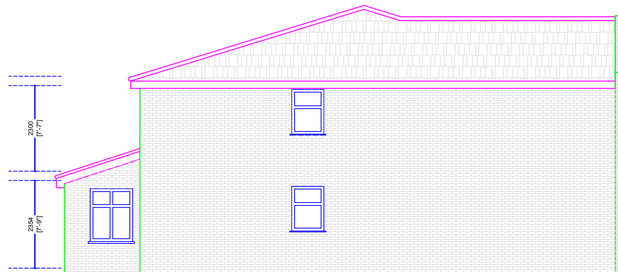
Proposed Side Elevation (North West)
