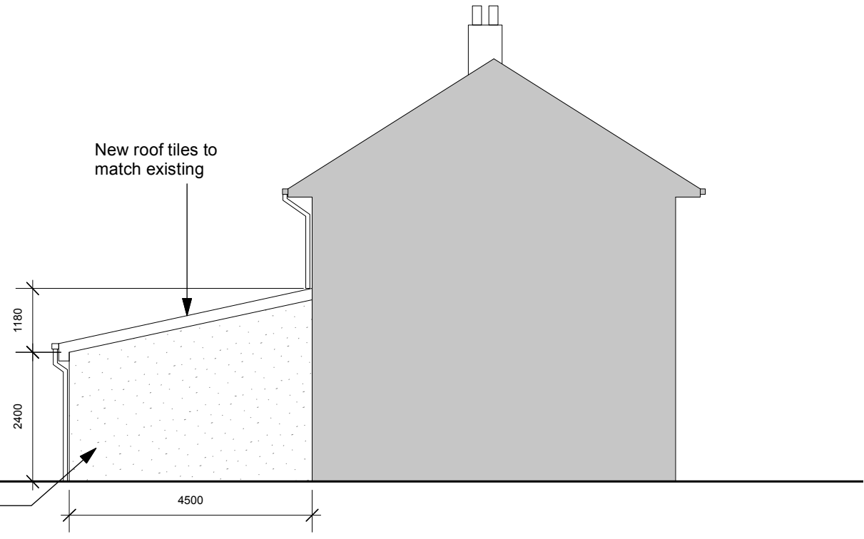
NORTH WEST (SIDE) ELEVATION
