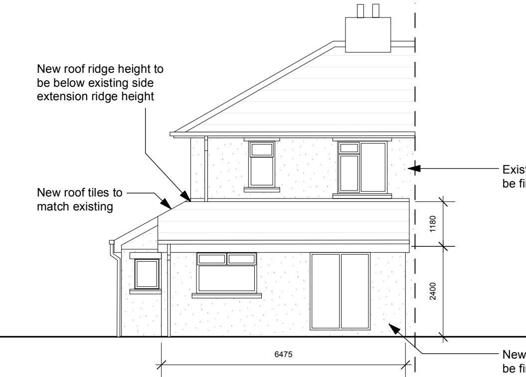
NORTH EAST (REAR) ELEVATION
