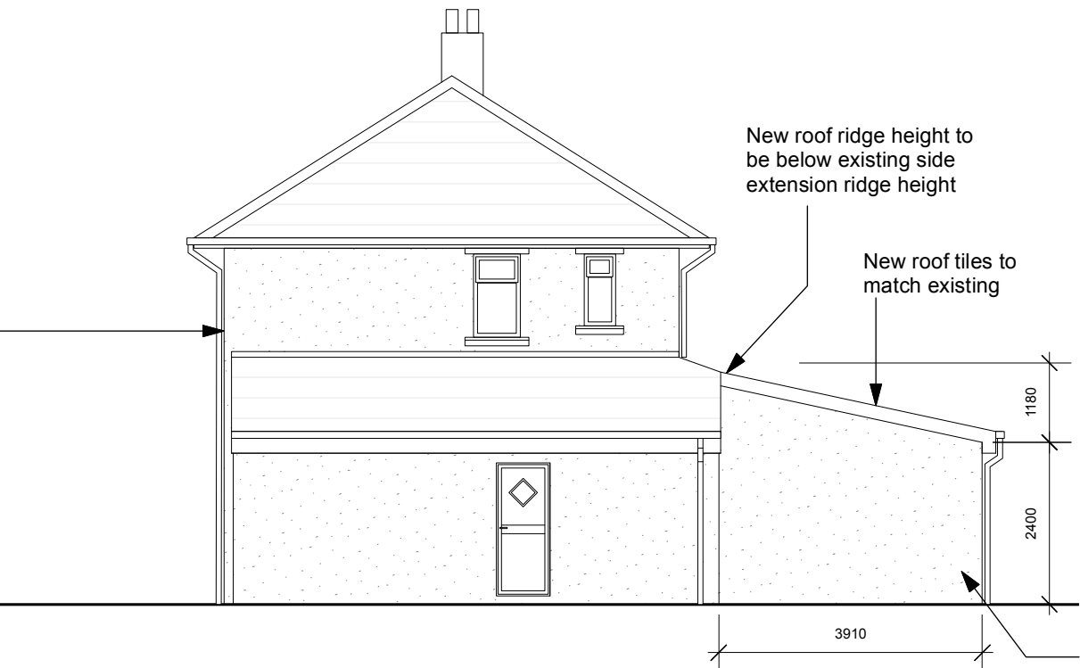
SOUTH EAST (SIDE) ELEVATION
