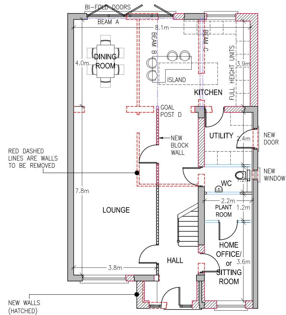
PROPOSED GROUND FLOOR PLAN 1:100 scale
