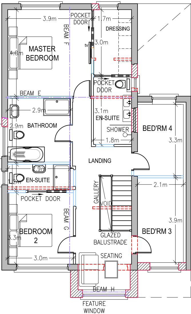
PROPOSED FIRST FLOOR PLAN 1:100 scale
