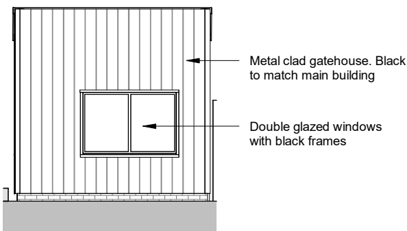
North Elevation
