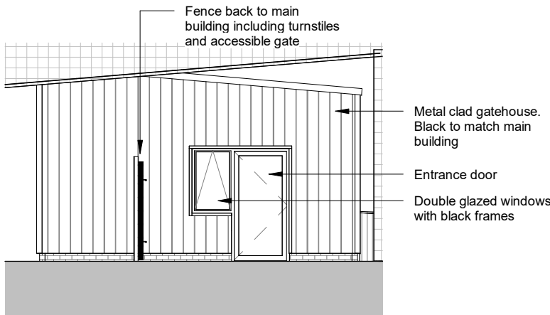
West Elevation
