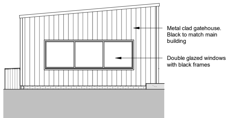
East Elevation
