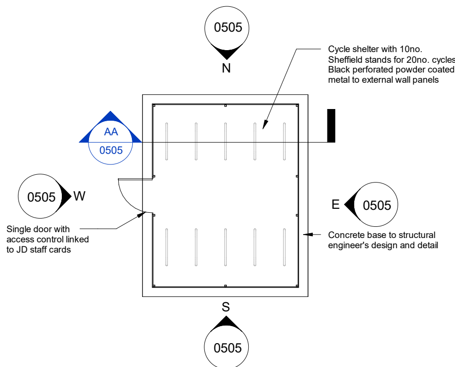
Proposed Floor Plan Scale @ 1 : 100
