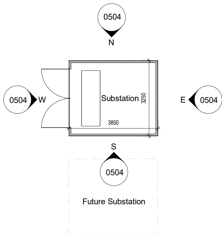
Proposed Floor Plan Scale @ 1 : 100
