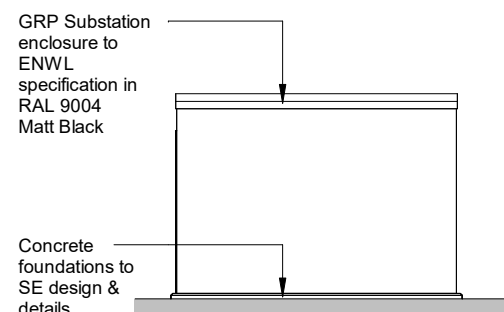
South Elevation Scale @ 1 : 100
