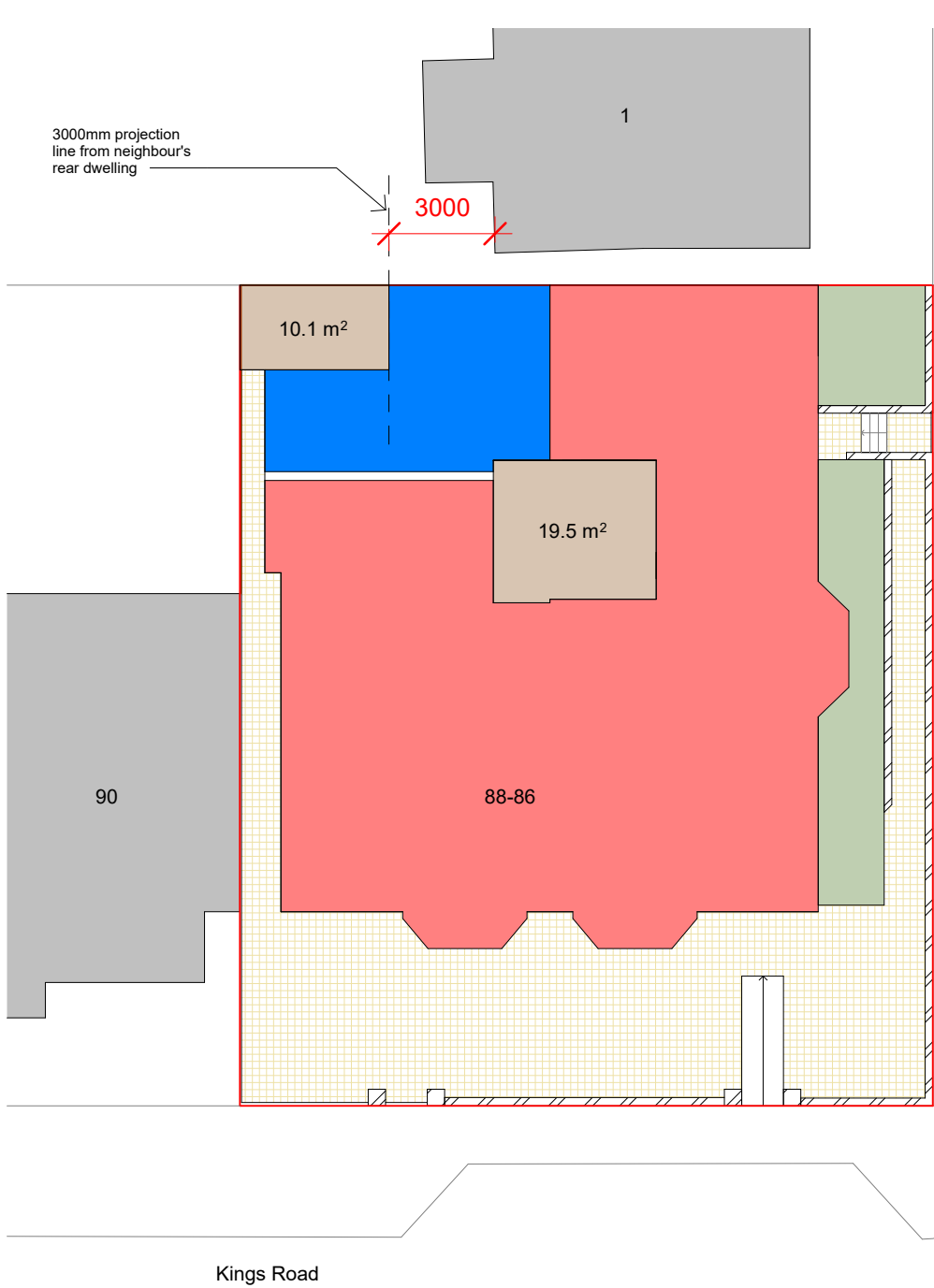
2 Site - Proposed 1 : 200
