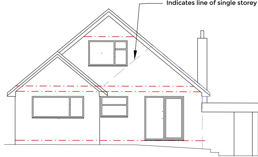
REAR ELEVATION 1:100
