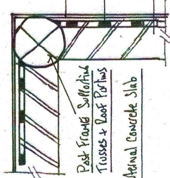
Plan View of Wall Construction
