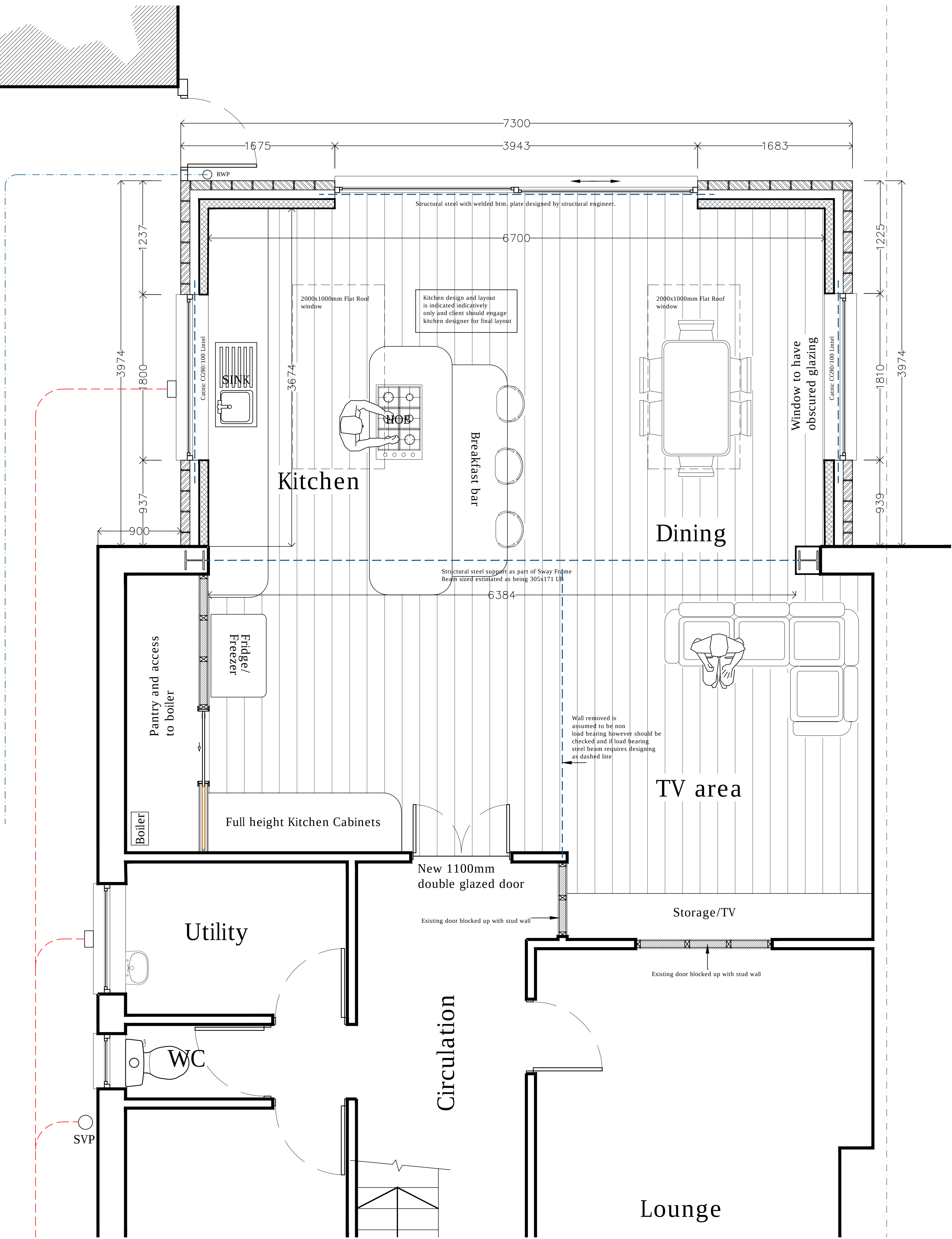
Proposed Part Ground Floor Plan (1:25)
