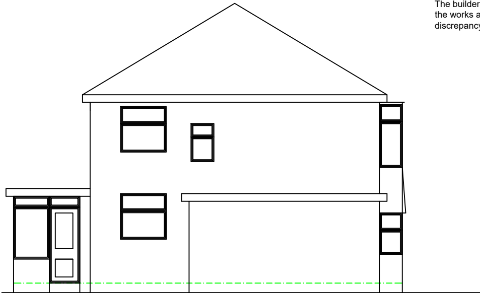
Side Elevation
