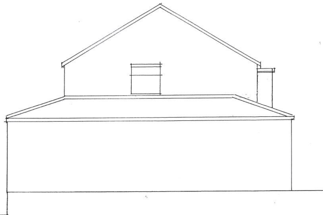
SOUTH ELEVATION
