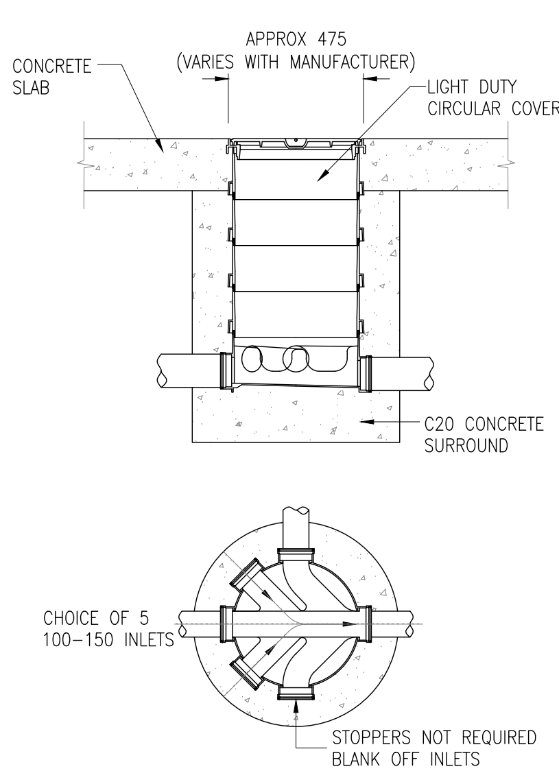
POLYPROPYLENE INSPECTION CHAMBER DETAILS
