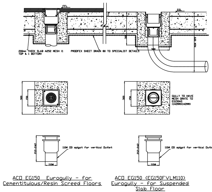
TYPICAL GULLY DETAIL FOR DEEP POP UP CONNECTIONS
