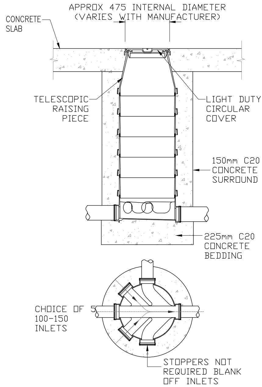
REDUCED ACCESS INSPECTION CHAMBER DETAILS (DEPTH 1.1m < 3m) (HARD LANDSCAPING)
