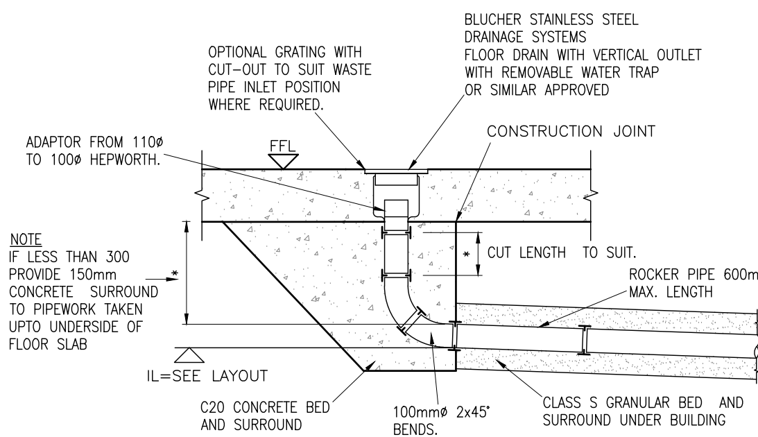
INTERNAL FLOOR DRAIN (1:20)
