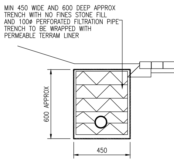
FILTER DRAIN DETAIL
