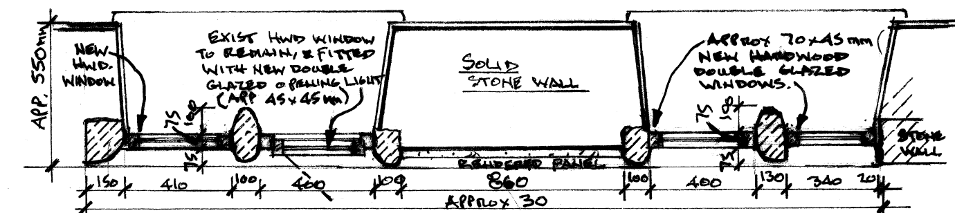
HORIZONTAL SECTION FRONT KITCHEN WINDOW. (3) 1:20.
