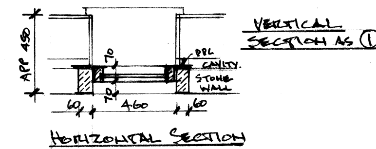
REAR PORCH/STUDY WINDOW (5)
