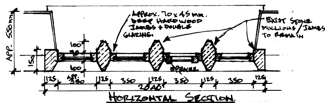
REAR LOUNGE WINDOW ①. 1:20.
