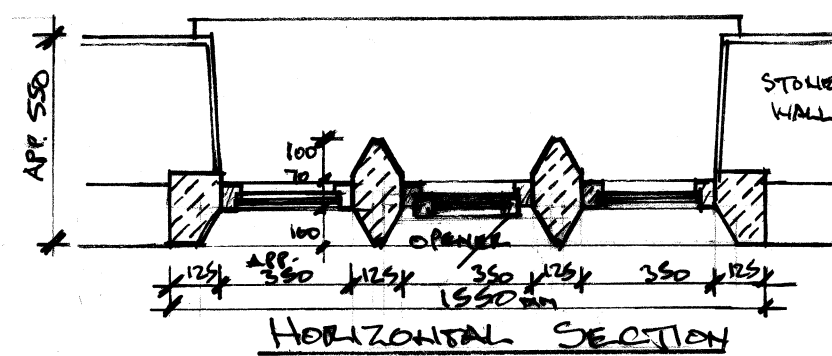
REAR BEDROOM WINDOW (2)
