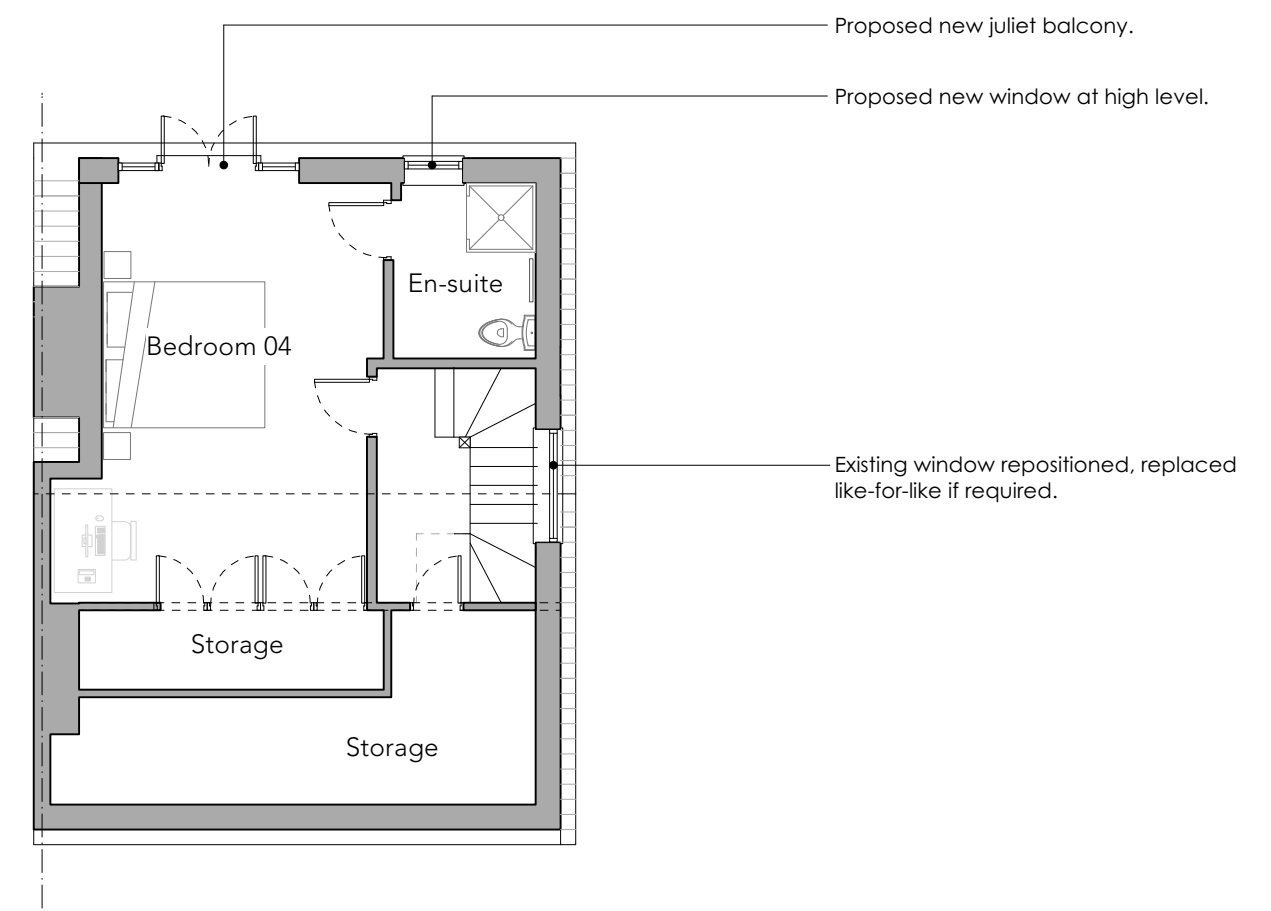
Proposed second floor plan 1:100
