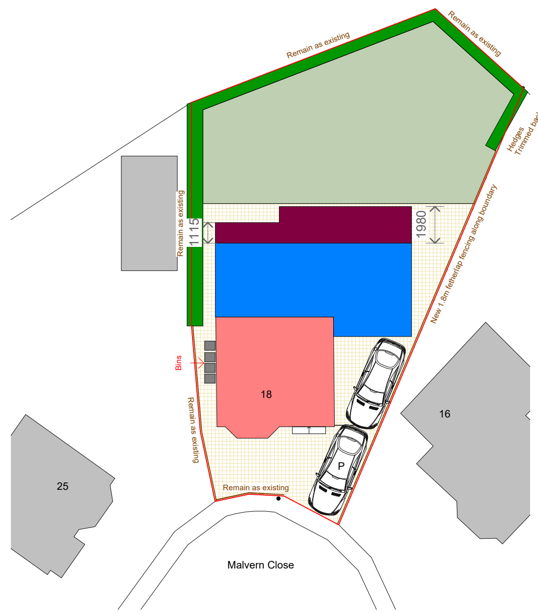
3 Site - Proposed (VOC) 1 : 200
