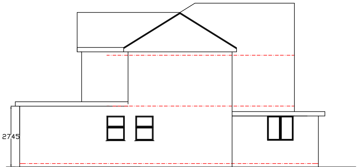
Side Elevation
