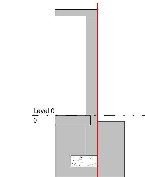
3 Foundation Section 1 : 50
