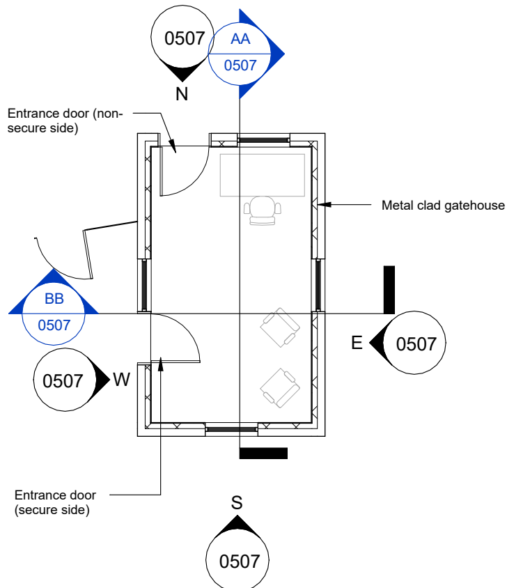
Proposed Floor Plan Scale @ 1 : 100
