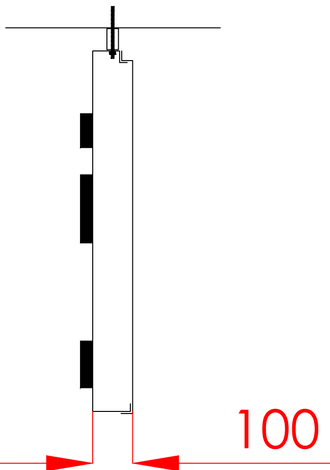
LETTER SECTION 1:10 @A1
