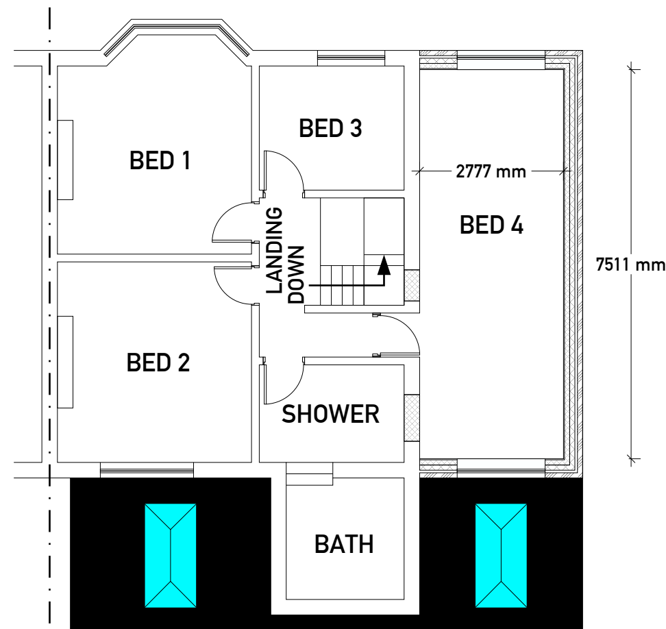
PROPOSED 1ST FLOOR PLAN WALL REMOVAL
