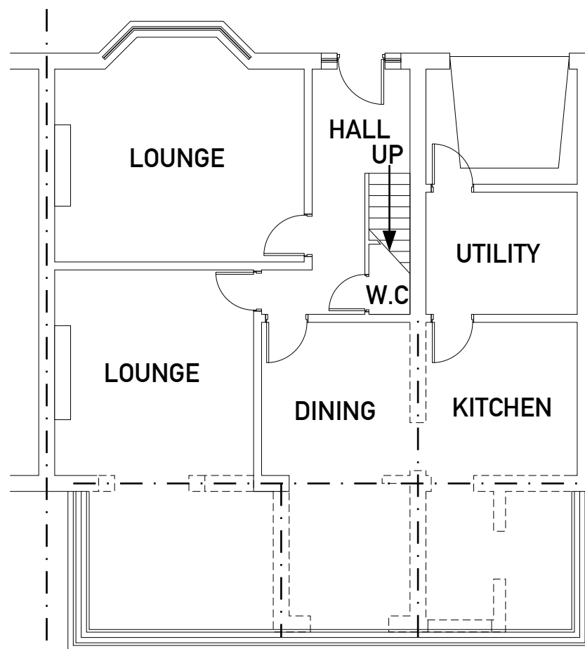
EXISTING GROUND FLOOR PLAN WALL REMOVAL
