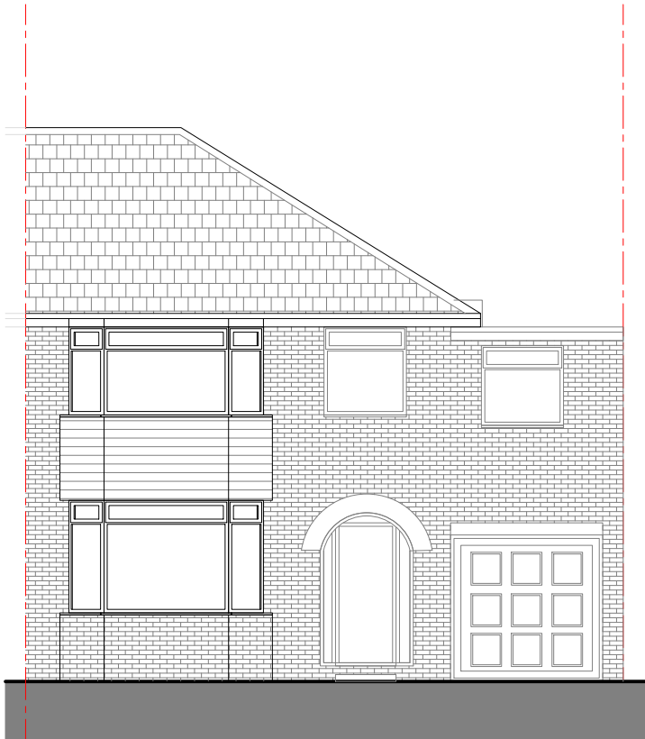
EXISTING FRONT ELEVATION 1:100 @ A3 0m 1m 3m 5m
