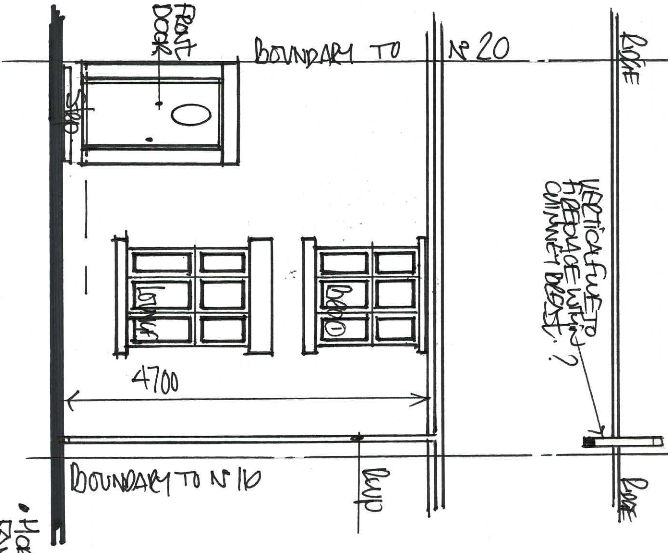
1:50 EXC "FRONT" ELEVATION
