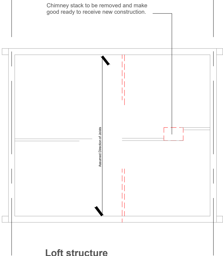
Loft structure
