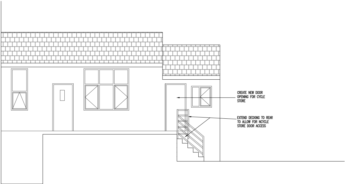
REAR SIDE ELEVATION AS PROPOSED
