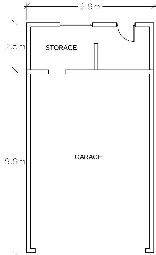
EXISTING OUTBUILDINGS PLAN (1:100)
