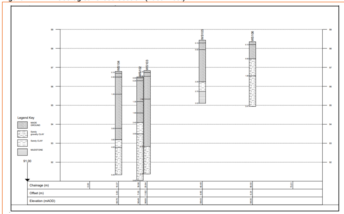
Figure 2 Geological Cross Section (East-West)
