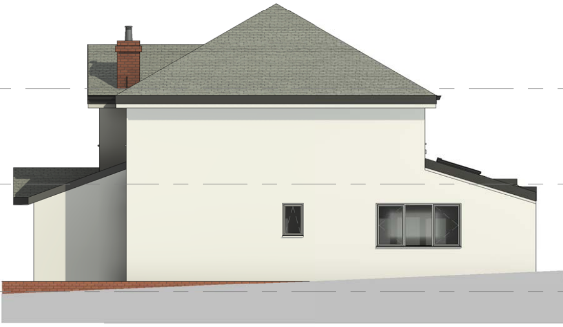
6. Right Side - Proposed 1 : 100
