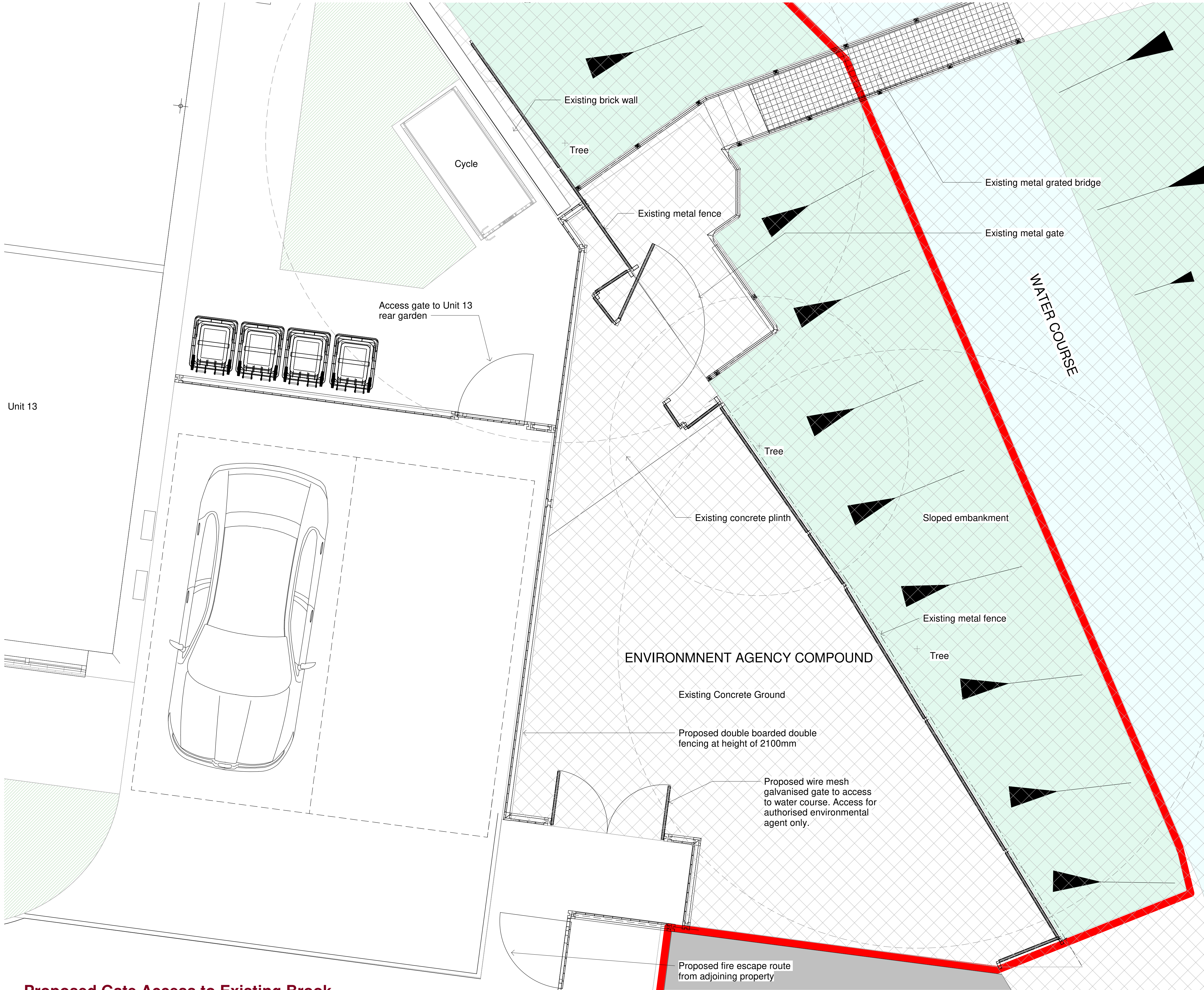
Proposed Gate Access to Existing Brook Scale 1 : 25
