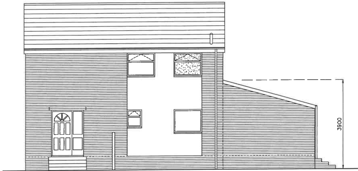
PROPOSED SOUTH EAST ELEVATION 1:100 @ A4
